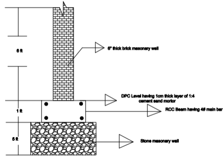
Section of wall
