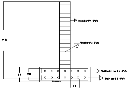
Section Column with footing
